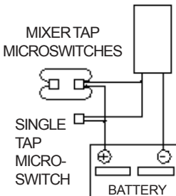
Fig. 3 Microswitch Wiring Diagram
