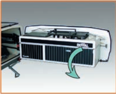
Swing the kitchen out and tilt down the wire clamp. See "kitchen section".
