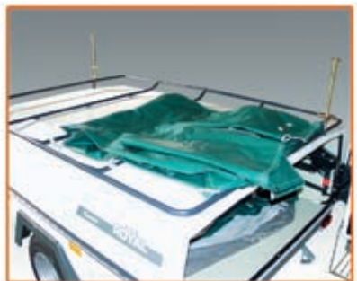
The under bed storage can be mounted before the lid is lifted over
